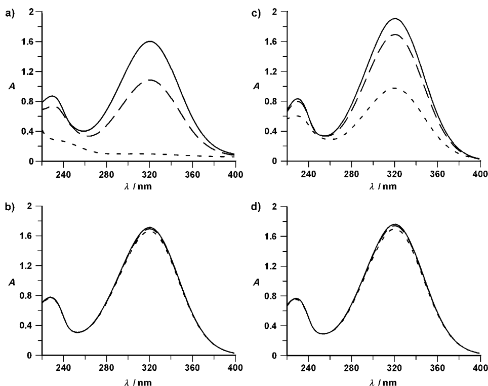
Figure 1. UV spectra showing the depletion of nitrostyrene ( 8 ) in the presence of a) acetaldehyde ( 7 ) and recombinant 4-OT, b) acetaldehyde ( 7 ) and synthetic 4-OT, c) acetaldehyde ( 7 ) and synthetic 4-OT, and d) recombinant 4-OT. — 0 min, --- 4 min, ..... 20 min.
